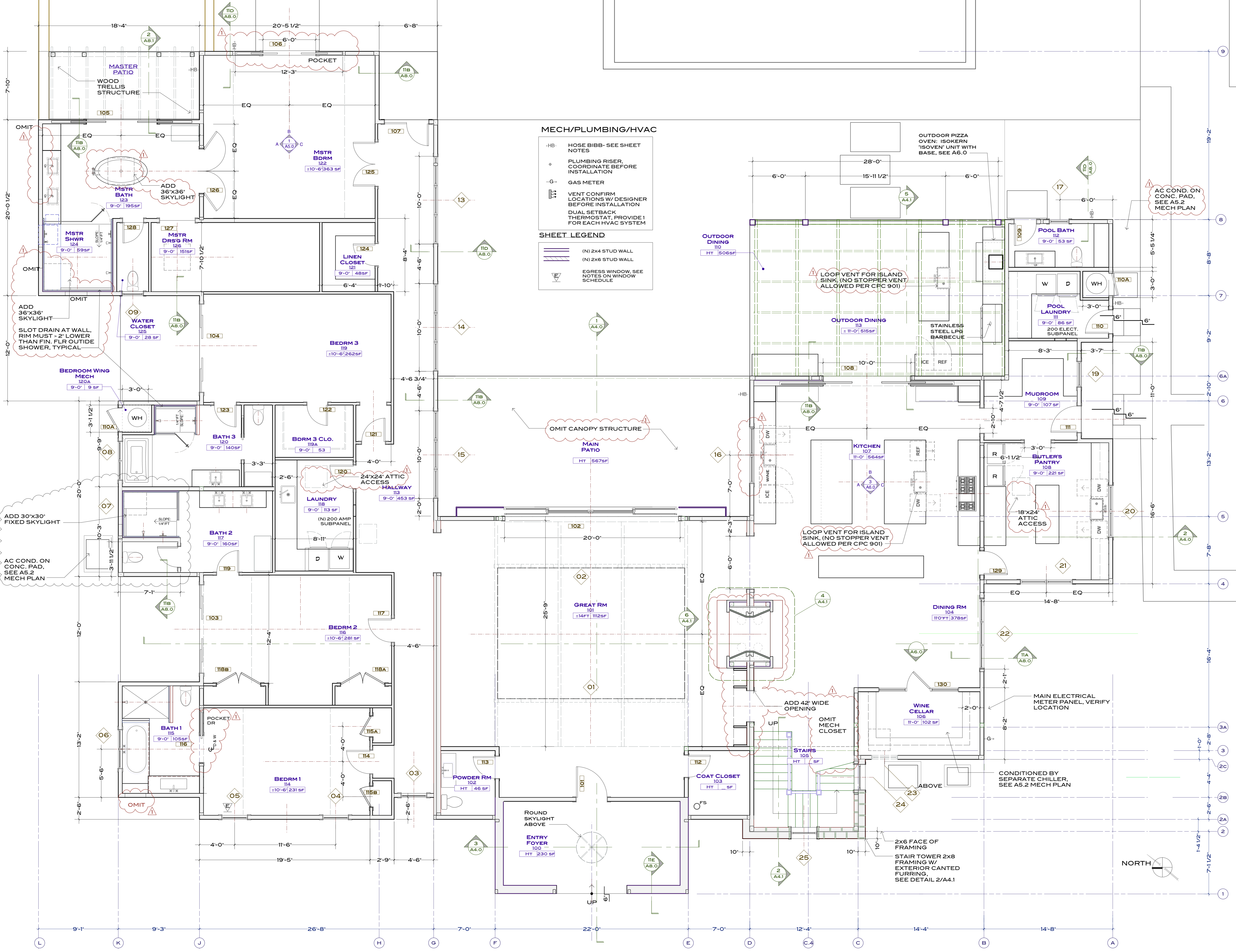
MAIN FLOOR PLAN 1 1/4" = 1'-0"
